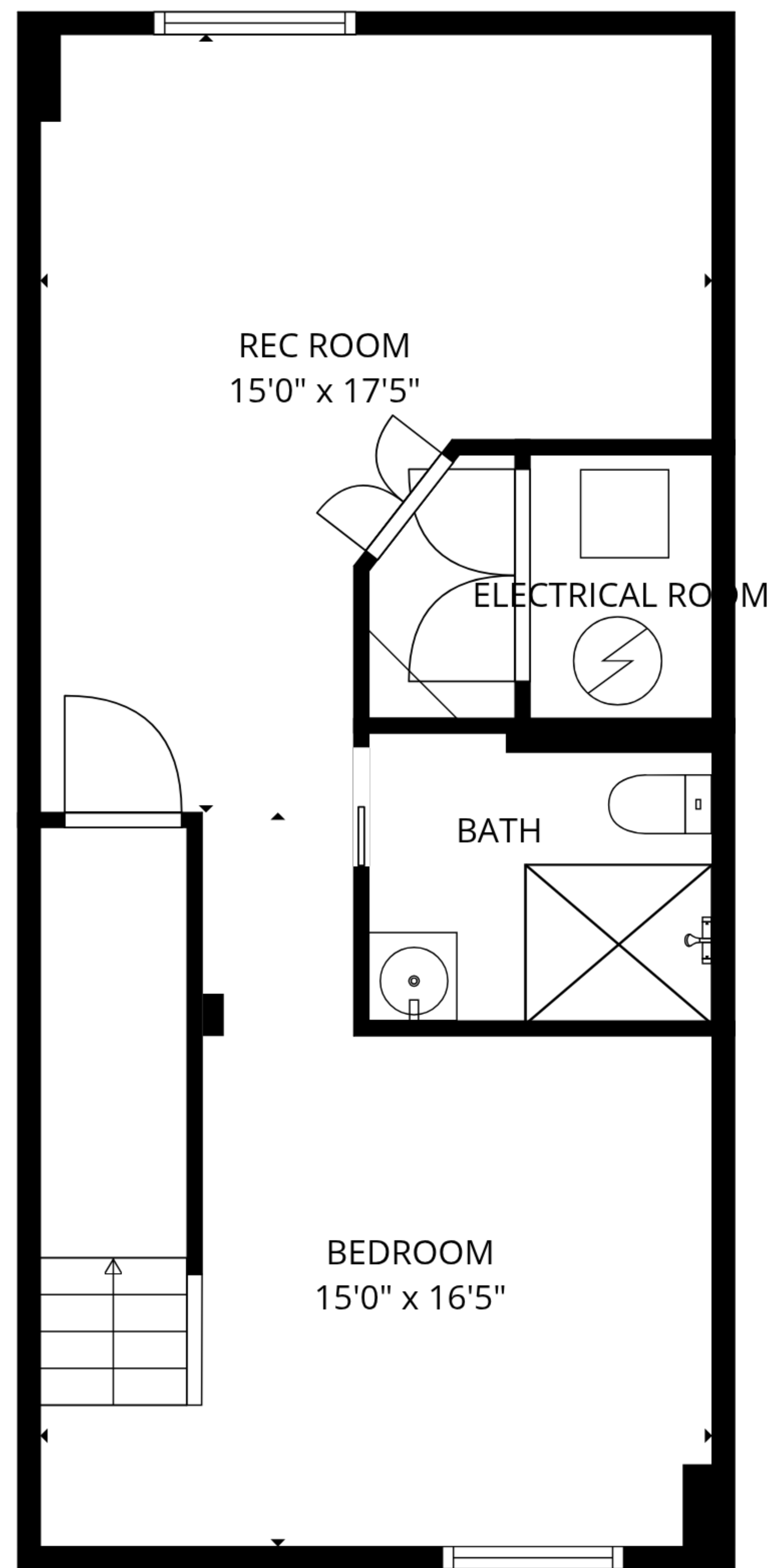
FLOOR 1
